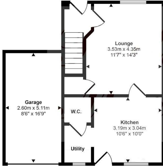
Ground Floor Approx 48 sq m / 518 sq ft
