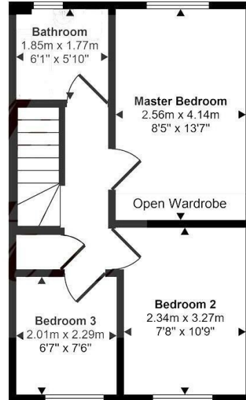
First Floor Approx 34 sq m / 368 sq ft
